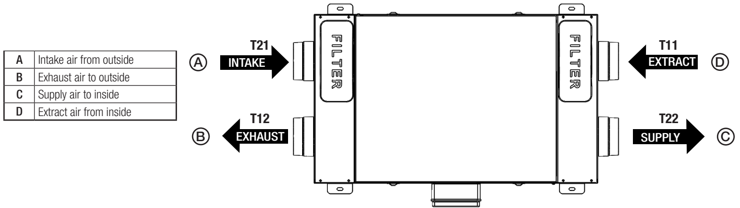
Fig.6.a Temperature probes
