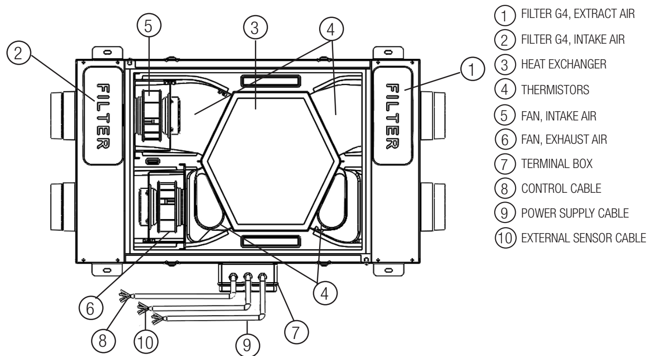
Fig. 7.a Internal components
