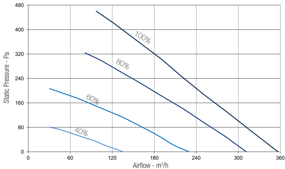
Fig.5.c Intake curve according to Reg. 1253/2014 (ErP).
