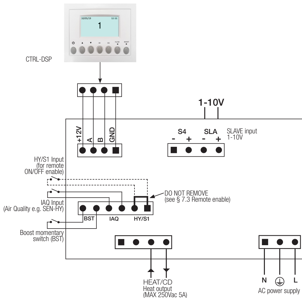
Fig. 4.g Electrical connections on the motherboard fitted in the terminal box.
